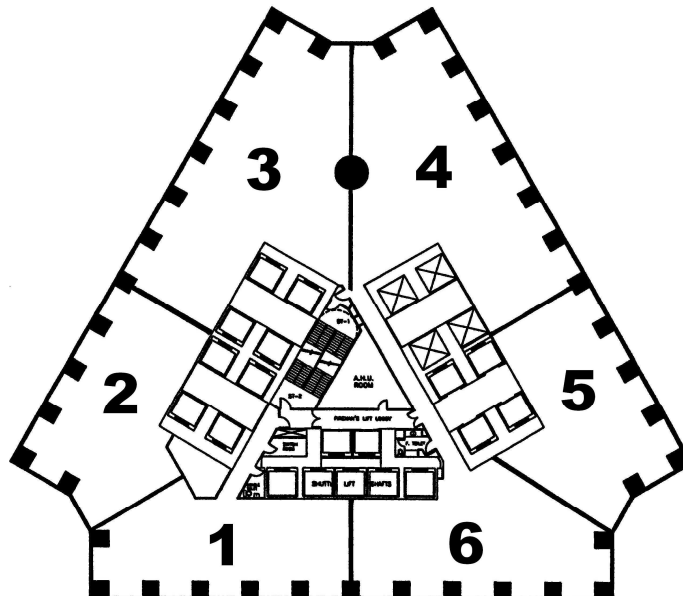
TYPICAL A/C ZONING PLAN CENTRAL PLAZA
